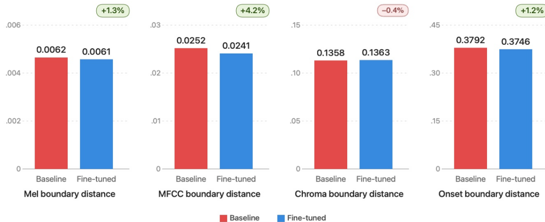
Figure 4 Baseline vs fine-tuned boundary distances.
